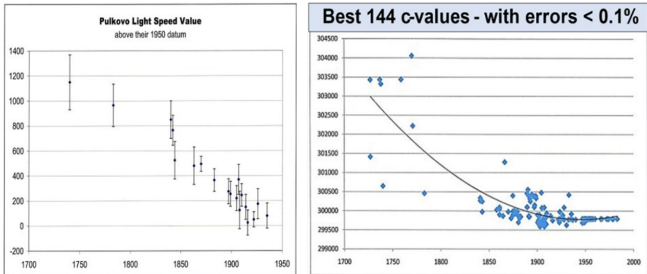
Figure 5: (Left) Light-Speed Determined by The Aberration Method at Pulkovo Observatory. (Right) c-values with Errors Less than 0.1%. Further Analysis and Explanations can be found in References 60 and 61.
