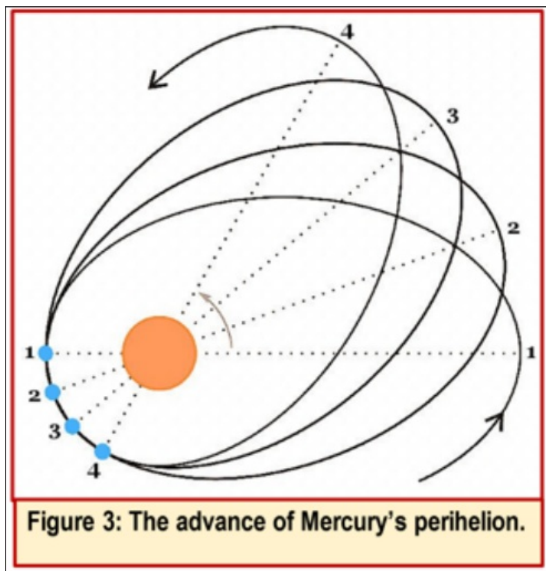
Figure 3 The advance of Mercury's perihelion
